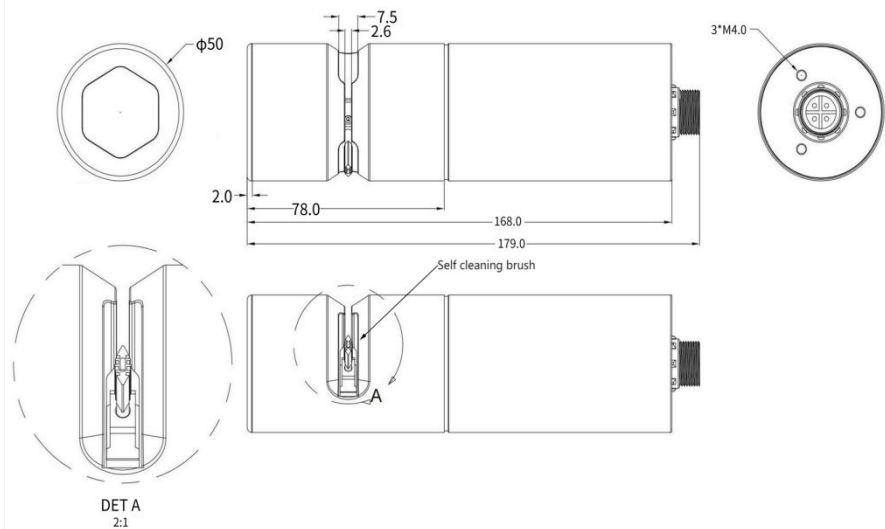
Fig.2 Regular large range COD sensor (Unit: mm)
