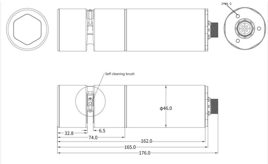
Fig.3 Economical type COD sensor (Unit: mm)
