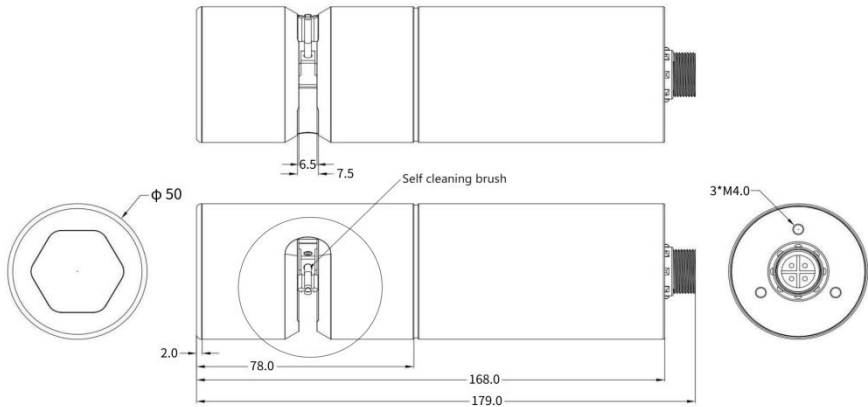
Fig.1 Regular small range COD sensor (Unit: mm)
